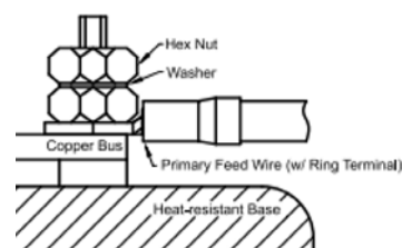
Recommended mounting
