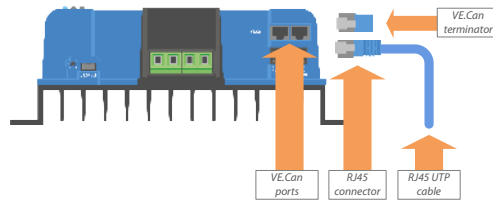
VE.Can port, connector, terminator and cable
